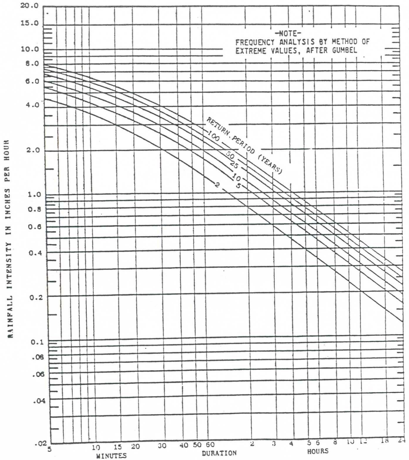
Figure 2.16 Rainfall Intensity-Duration-Frequency Curves Evansville, Indiana 1903 - 1951
