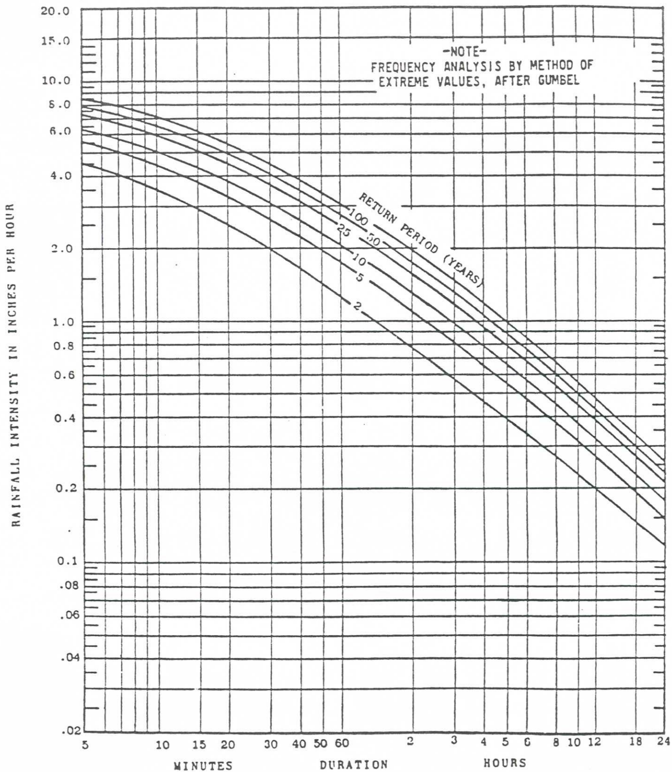
Figure 2.17 Rainfall Intensity-Duration-Frequency Curves Indianapolis, Indiana 1903 - 1951
