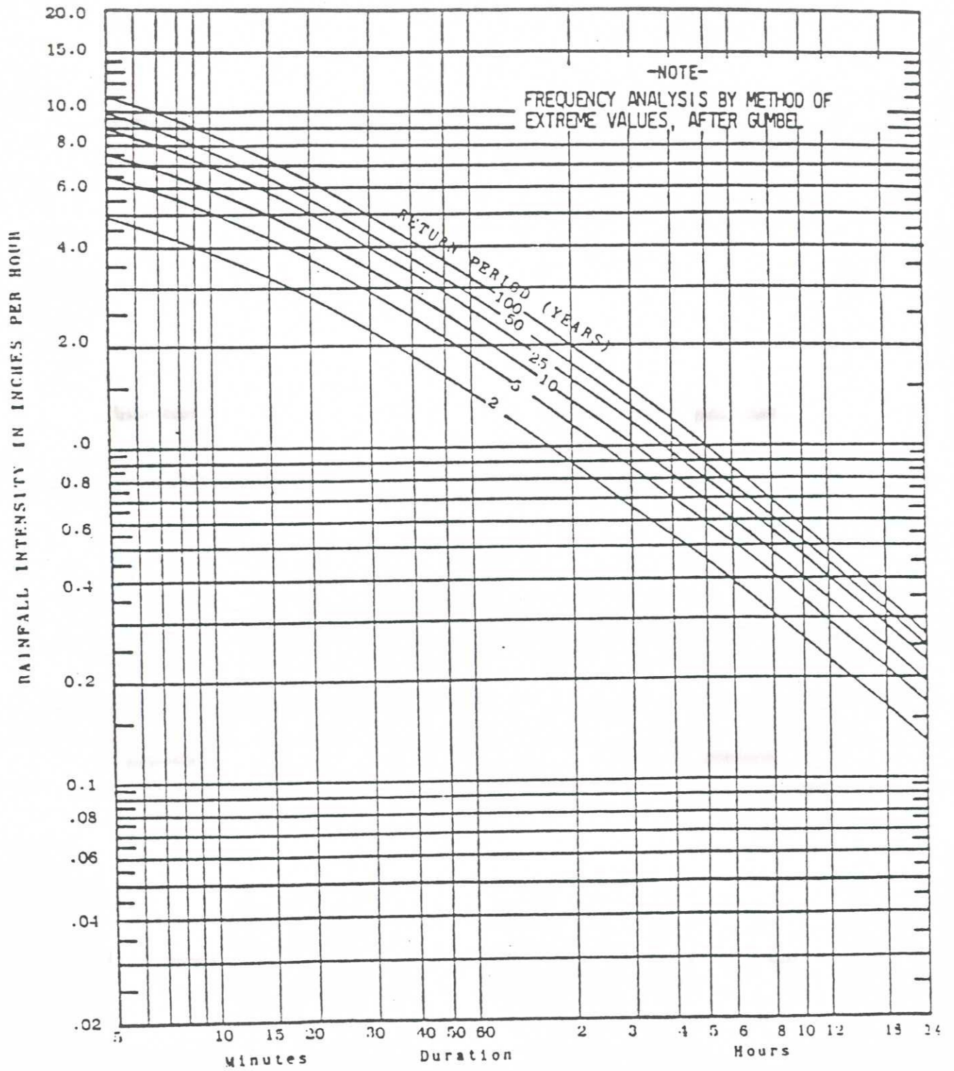
Figure 2.18 Rainfall Intensity-Duration-Frequency Curves Terre Haute, Indiana 1912 - 1951
