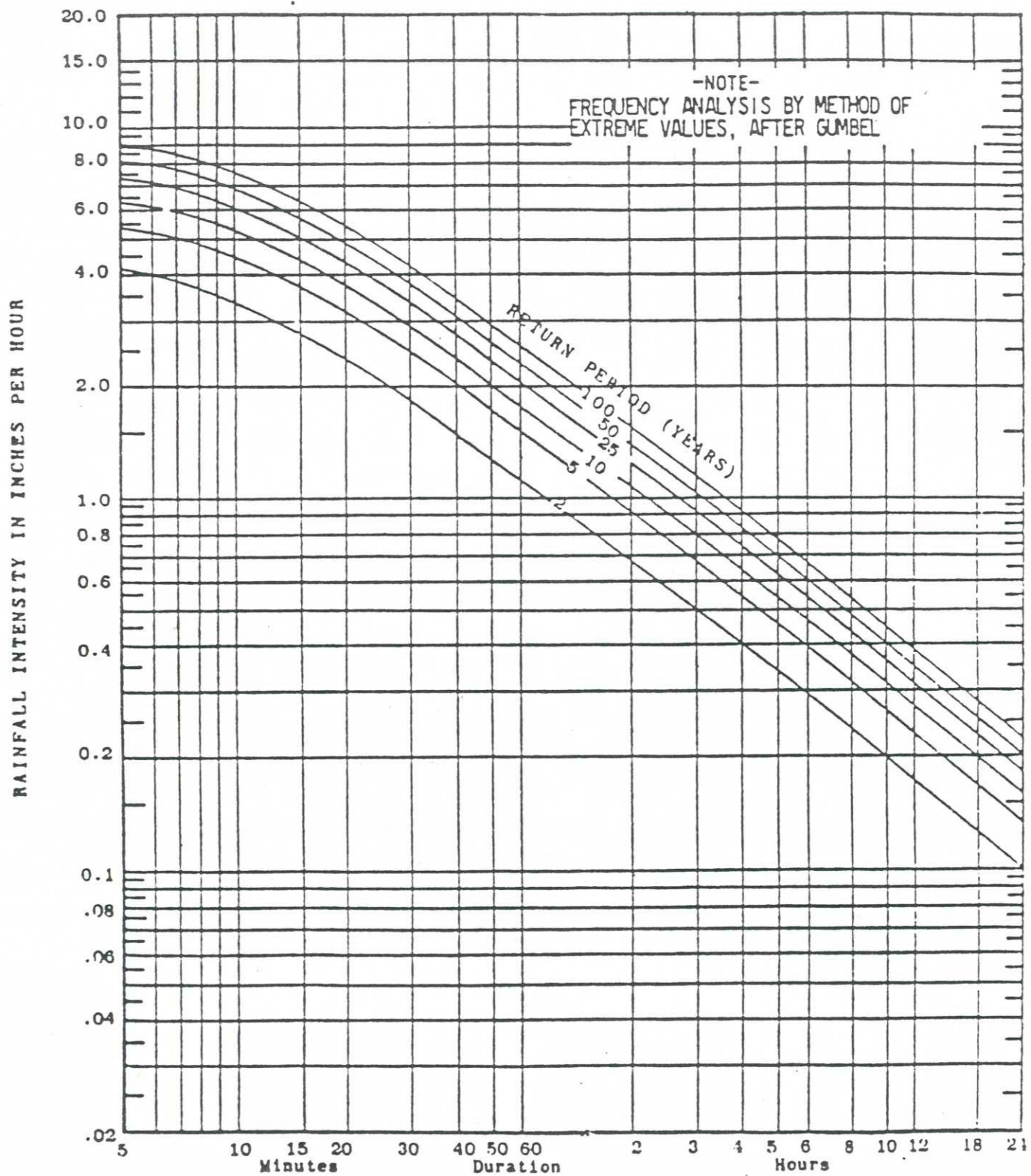
Figure 2.15 Rainfall Intensity-Duration-Frequency Curves
