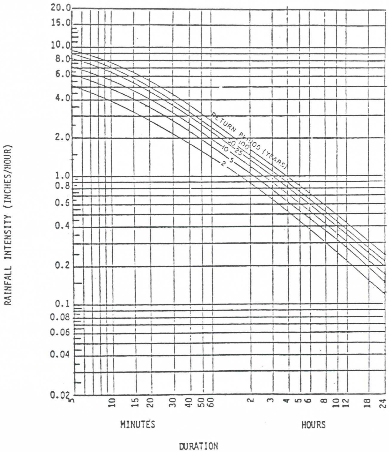
Figure 2.20 Rainfall Intensity-Duration-Frequency Curves West Lafayette, Indiana (Burke, 1979)
