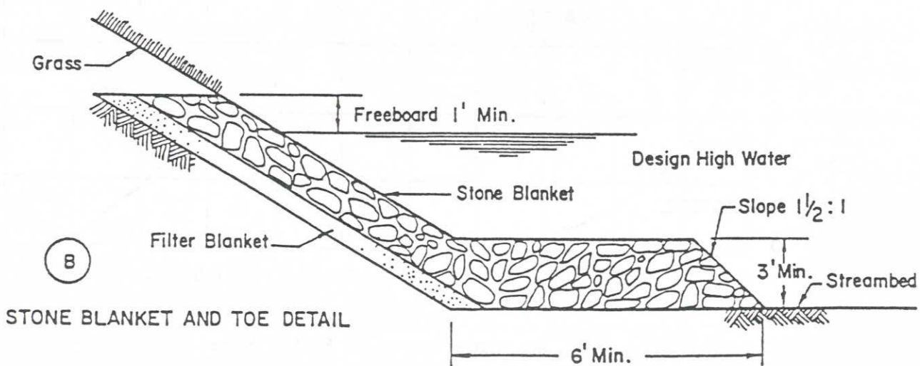
STONE BLANKET AND TOE DETAIL
