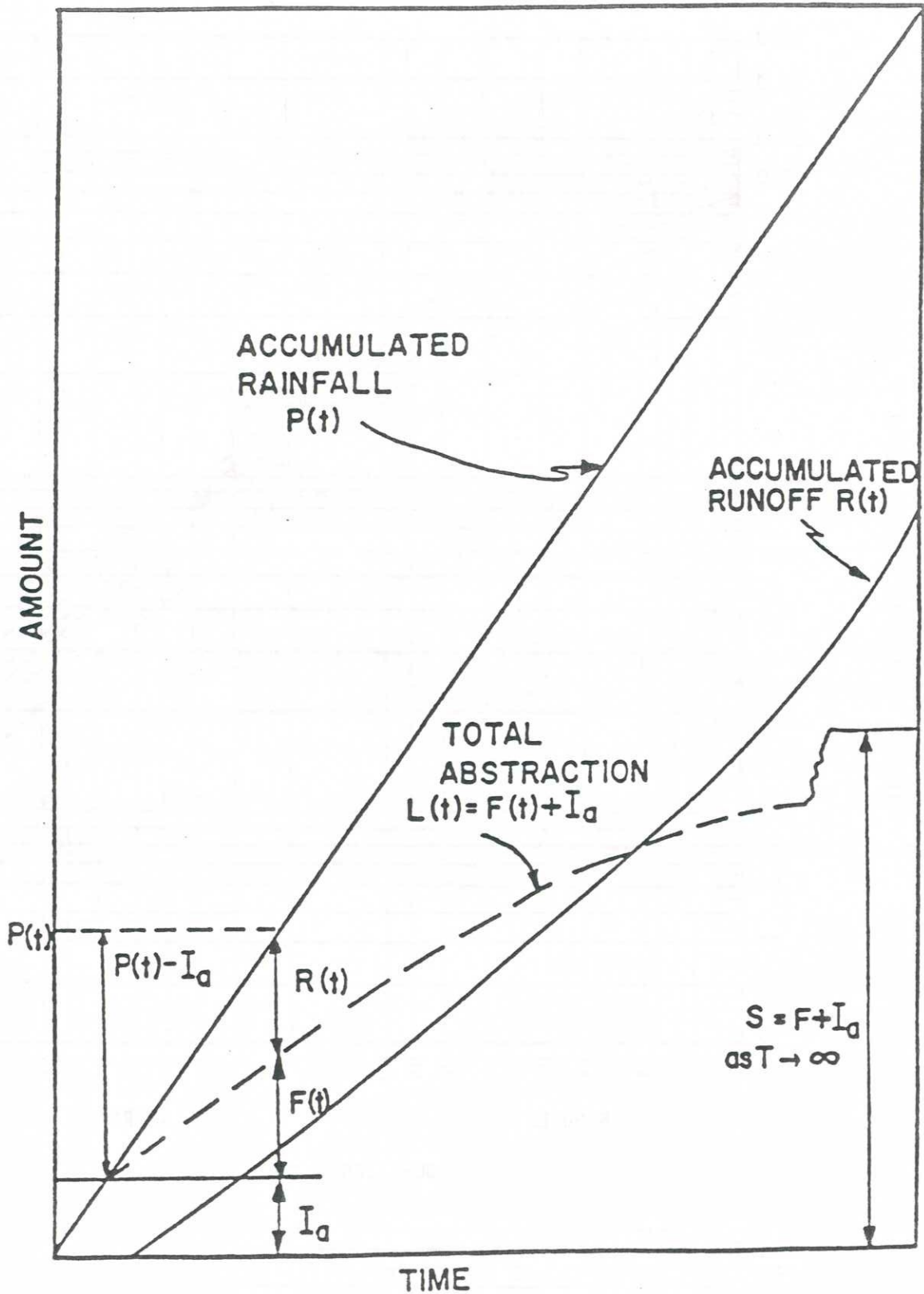
SCS CURVE NUMBER DIAGRAM OF ACCUMULATED RAINFALL, RUNOFF & INFILTRATION
