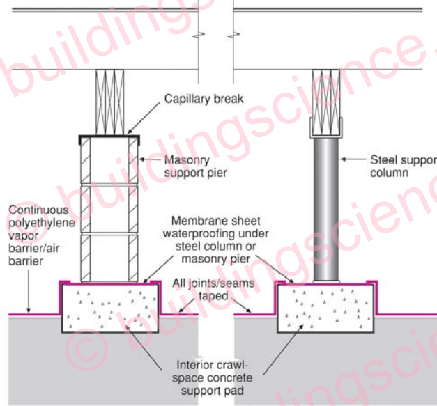
Figure 8 Air Barrier Continuity at Piers
